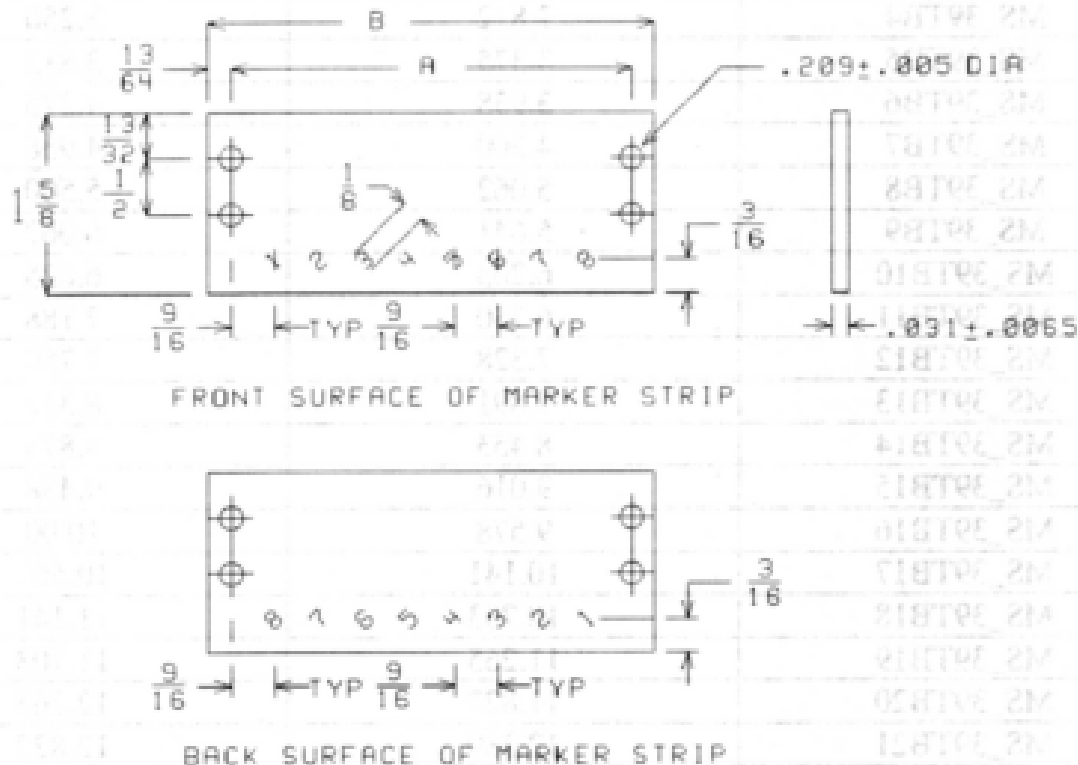
Figure 1. Terminal Board Marker Strip, Type MSA39TB8.
