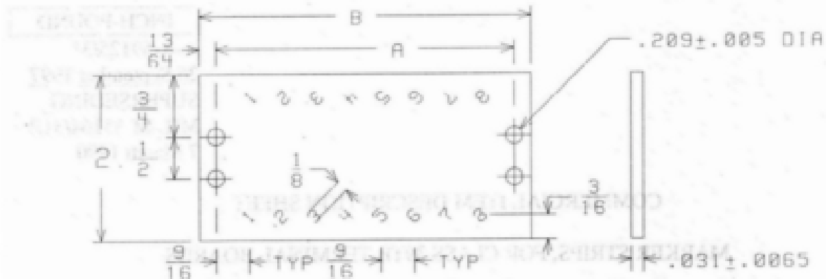
Figure 2. Terminal Board Marker Strip, Type MSA39TB8.
